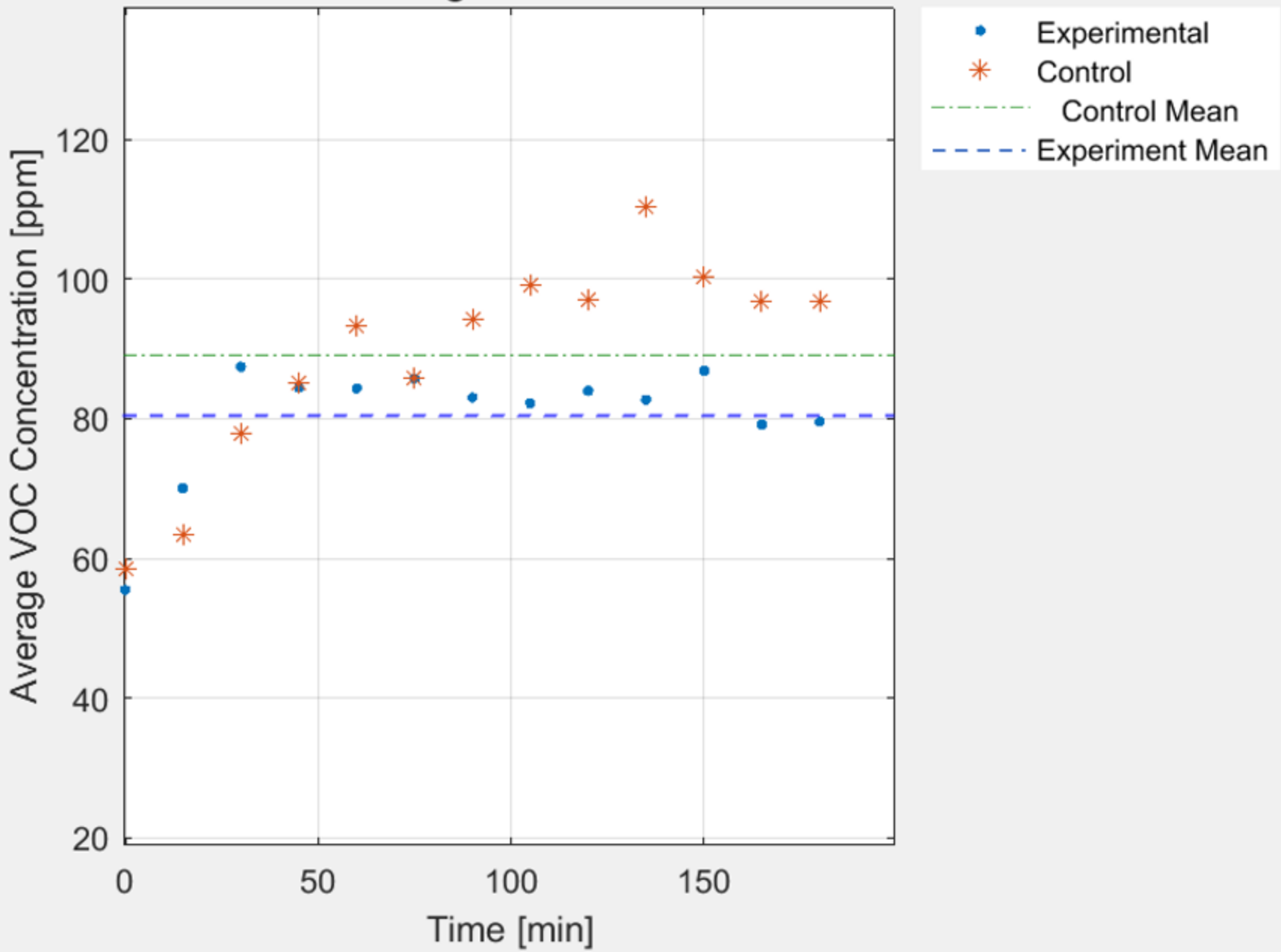
Time vs. Average VOC Concentration
