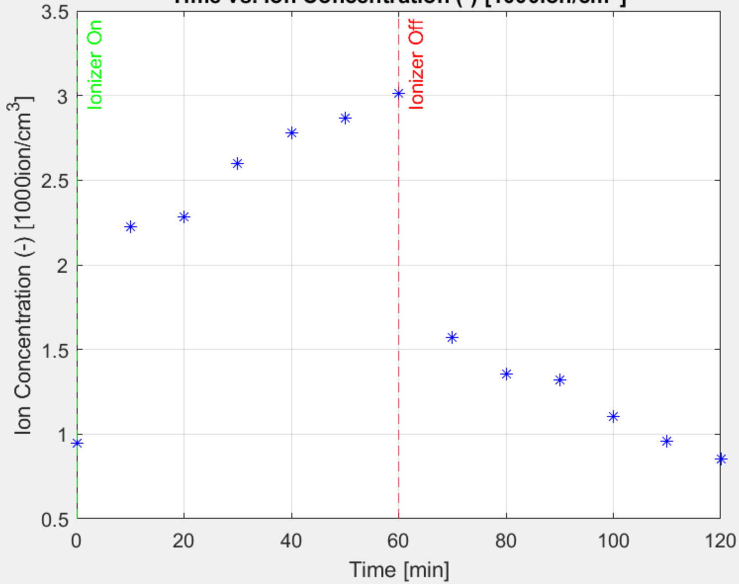
Time vs. Ion Concentration (-) [1000ion/cm 3 ]
