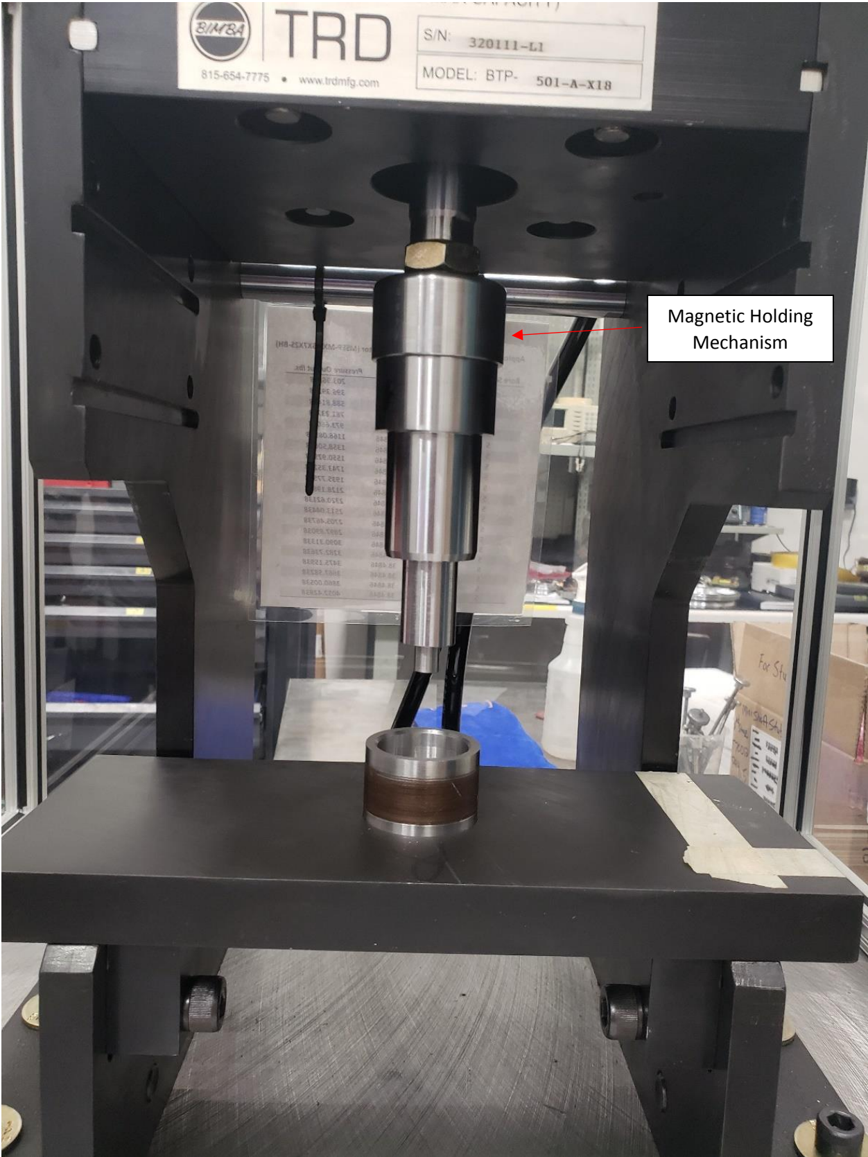
Shaft loaded into magnetic holding mechanism, aligned with radial sensor
